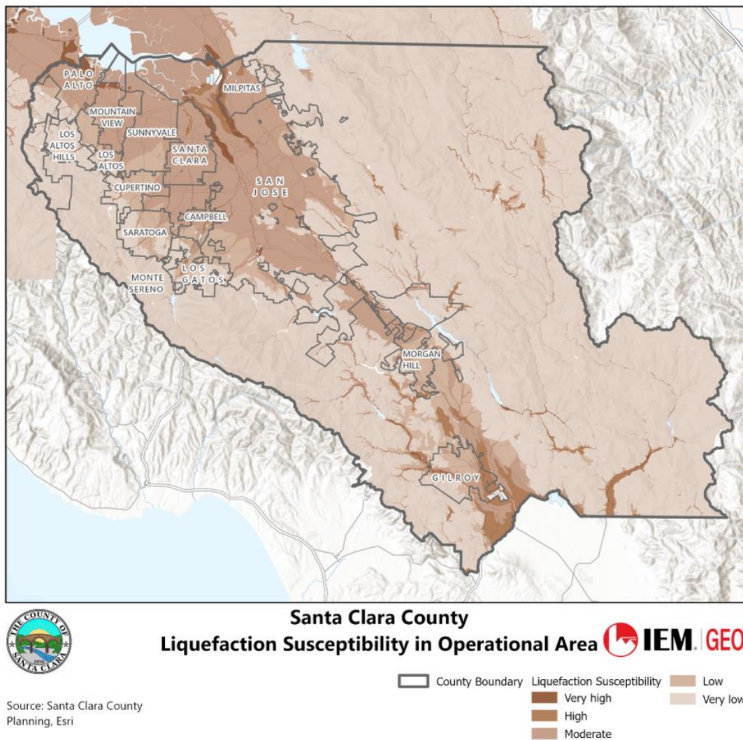
Figure 28: Liquefaction Susceptibility
